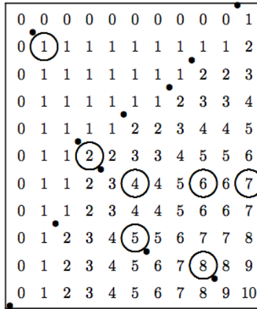
FIGURE 6. An example of admissible partial transposition.
